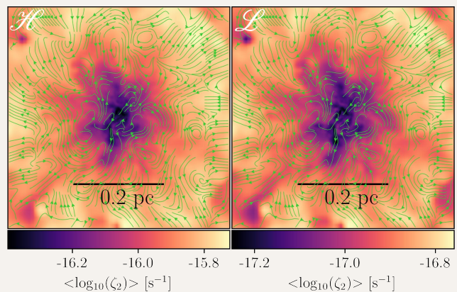
Fig. 1: Cosmic-ray ionization rate maps.
