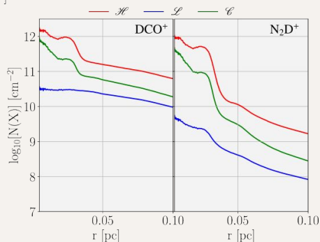
Fig. 2: Radial profiles of N(\text{DCO}^+) and N(\text{N}_2\text{D}^+) .
